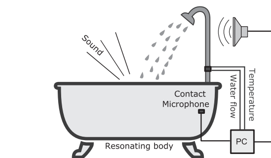
Figure 1: Hardware setup of our auditory display: Based on the current water flow and temperature data, the sound that is picked up by the contact microphone is processed and, through a speaker, directly fed back to the user.
